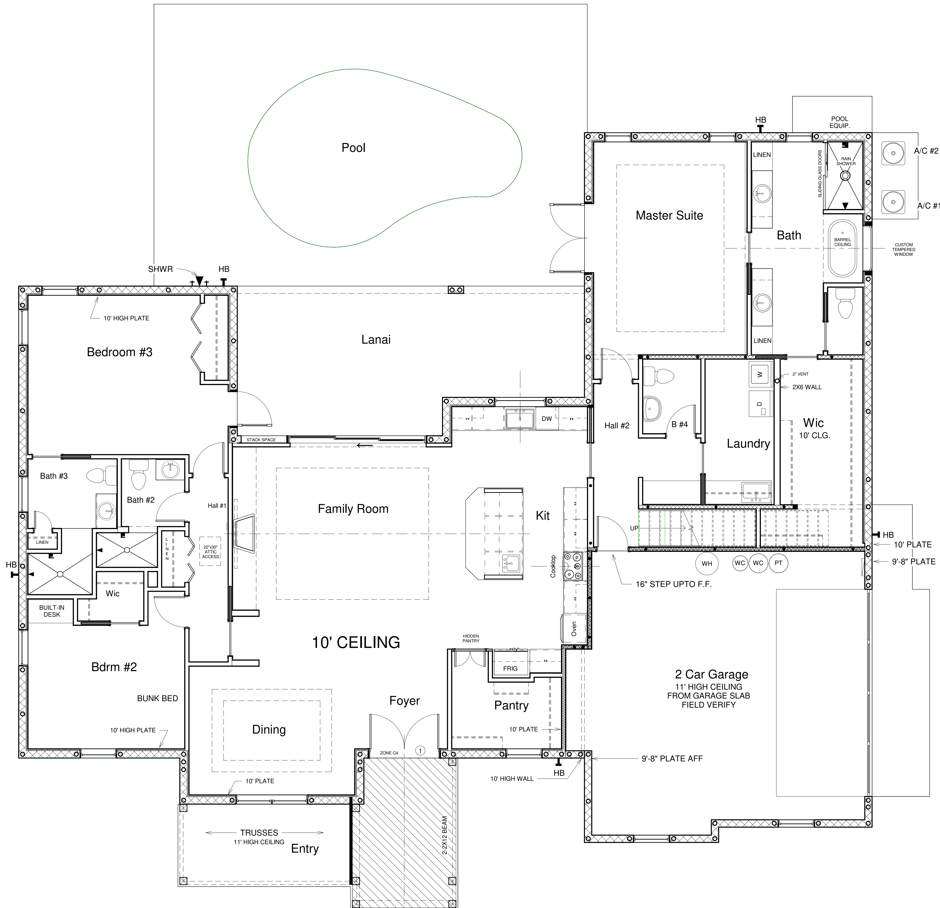
1 Brochure Ground Floor 1/4" = 1'-0"
